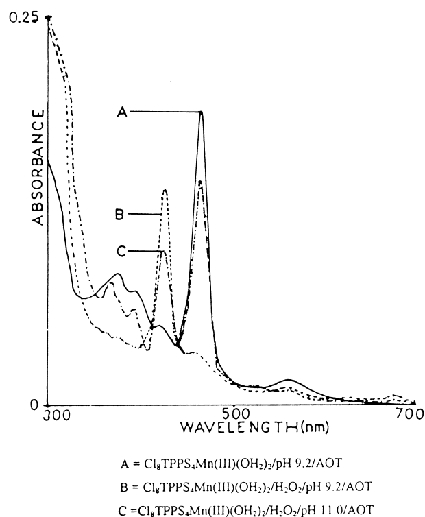
Figure 1. Formation of high valent oxo -manganese(IV) radical cation from the reaction of \text{H}_2\text{O}_2 with \text{Cl}_8\text{TPPS}_4\text{Mn(III)Cl} ( 1 ) in AOT reverse micelle at different pH. All the reactions were performed at -40^\circ\text{C} in phosphate buffer (pH 7.0, 9.2 and 11.0). \text{Cl}_8\text{TPPS}_4\text{Mn(III)Cl} , 1.8 \times 10^{-7} mol; \text{H}_2\text{O}_2 , 1.0 \times 10^{-5} mol; AOT, 3 \text{ cm}^3 .
