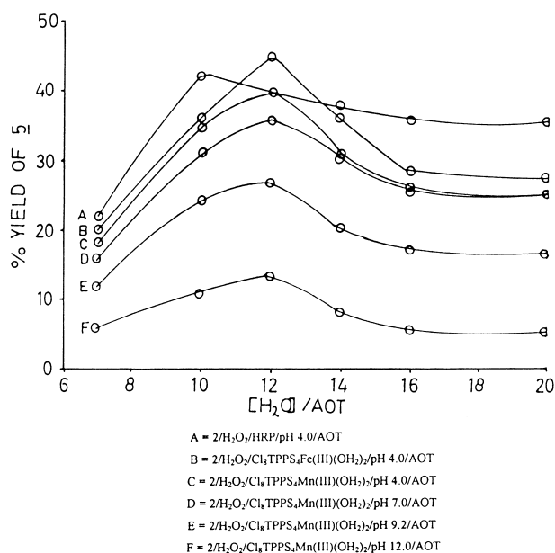
Figure 2. Formation of 5 from 2 and \text{H}_2\text{O}_2 catalyzed by HRP and water soluble porphyrins in AOT reverse miscelles at different pH and water:surfactant ratio, \text{Wo} . All the reactions were performed at room temperature in acetate buffer (pH 4.0), phosphate buffer (pH 7.0, 9.2 and 12). \text{Cl}_8\text{TPPS}_4\text{Mn(III)Cl} , 1.8 \times 10^{-7} mol; \text{Cl}_8\text{TPPS}_4\text{Fe(III)Cl} , 1.9 \times 10^{-7} mol; \text{H}_2\text{O}_2 , 1.0 \times 10^{-5} mol; AOT, 3 \text{ cm}^3 .
